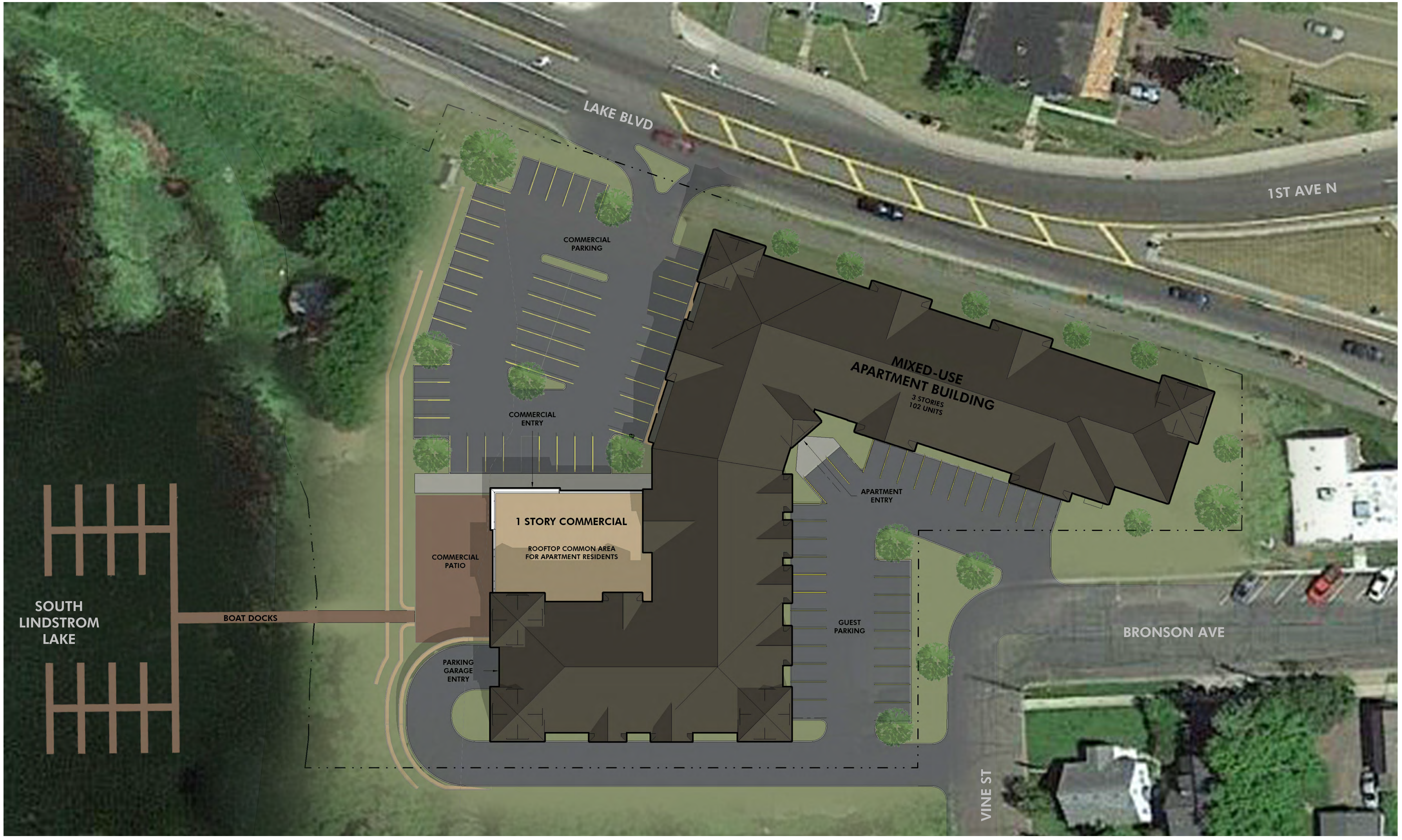
1 Colored Site Plan 1" = 20'-0"
